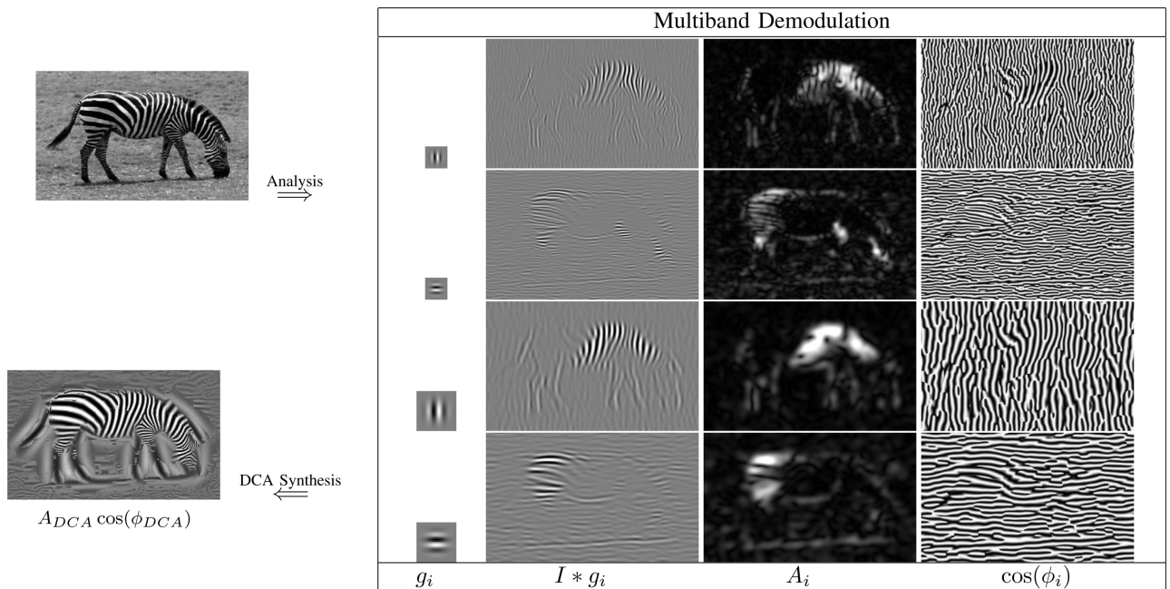
Fig. 4. The Dominant Component Analysis method for a locally narrowband signal: A set of bandpass Gabor filters is initially used to isolate and demodulate the individual components of (3). The dominant channel is subsequently chosen at each image location and its AM-FM parameters are used as a local texture descriptor. The principal structure of the textured signal is thus captured by the DCA parameters.
