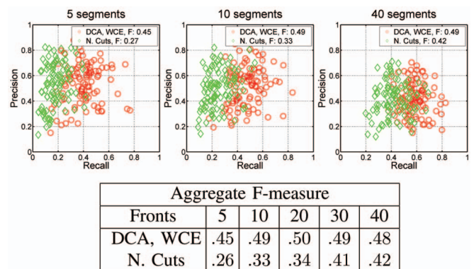
Fig. 11. Precision-Recall results on the Berkeley Benchmark obtained for an increasing number of image segments.
